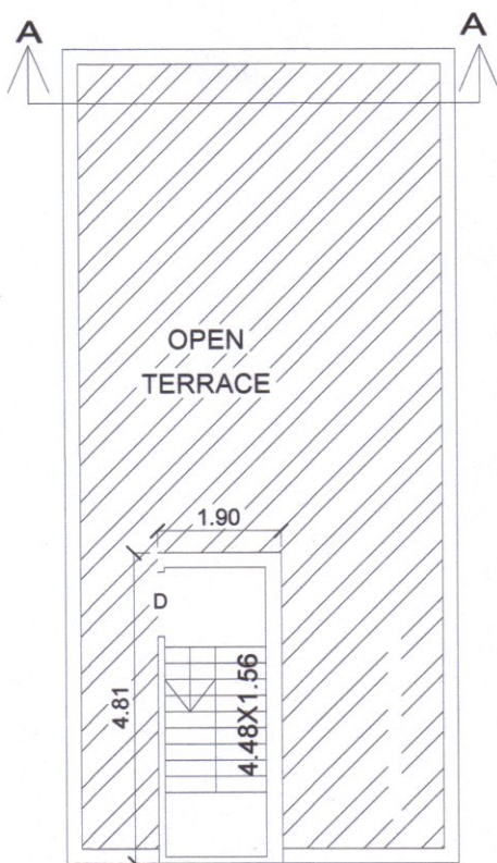
PLAN OF TERRACE FLOOR
