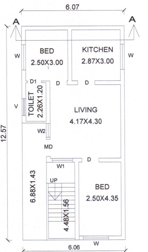
PLAN OF GROUND FLOOR
