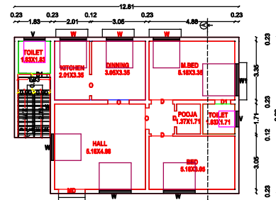
PROPOSED GF. PLAN
