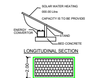
SOLAR SYSTEM
