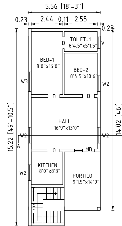
GROUND FLOOR BUILDING (EAST FACING BUILDING)
