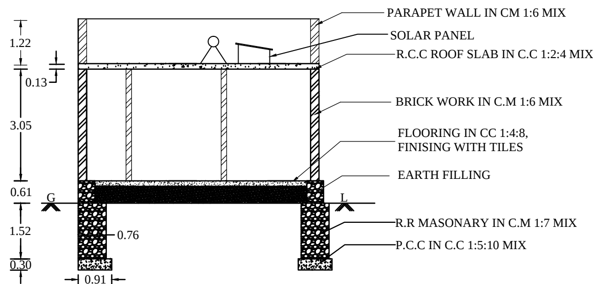
SECTION "A-B"
