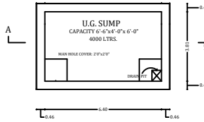
SUMP DETAIL
