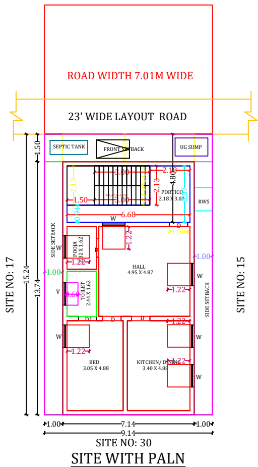
SITE PLAN
