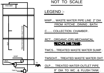
DETAILS OF WASTE WATER RECYCLING TANK, KITCHEN, DINING WASTE WATER REUSE METHOD NOT TO SCALE
