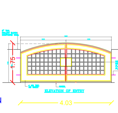
WIKET GATE ELEVATION
