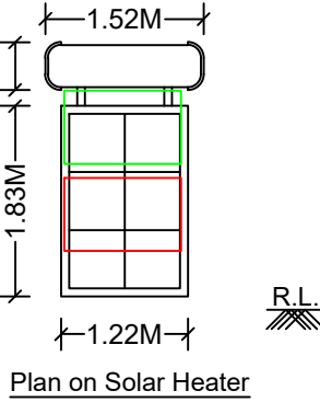
Plan on Solar Heater
