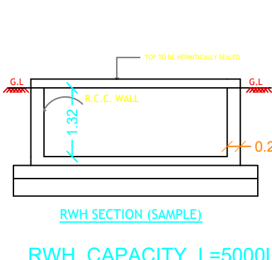
RWHT_CAPACITY_L=5000LTRS
