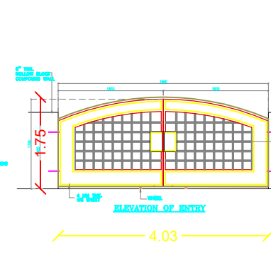
ELEVATION OF ENTRY
