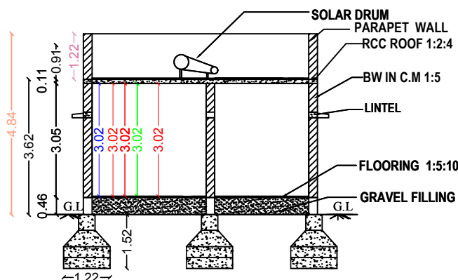
SECTION ON"AA"
