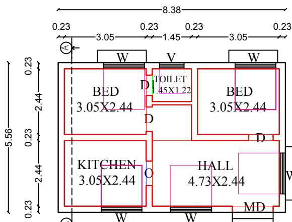
PROPOSED GF.PLAN
