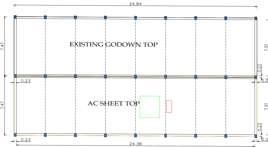
TERRACE FLOOR
