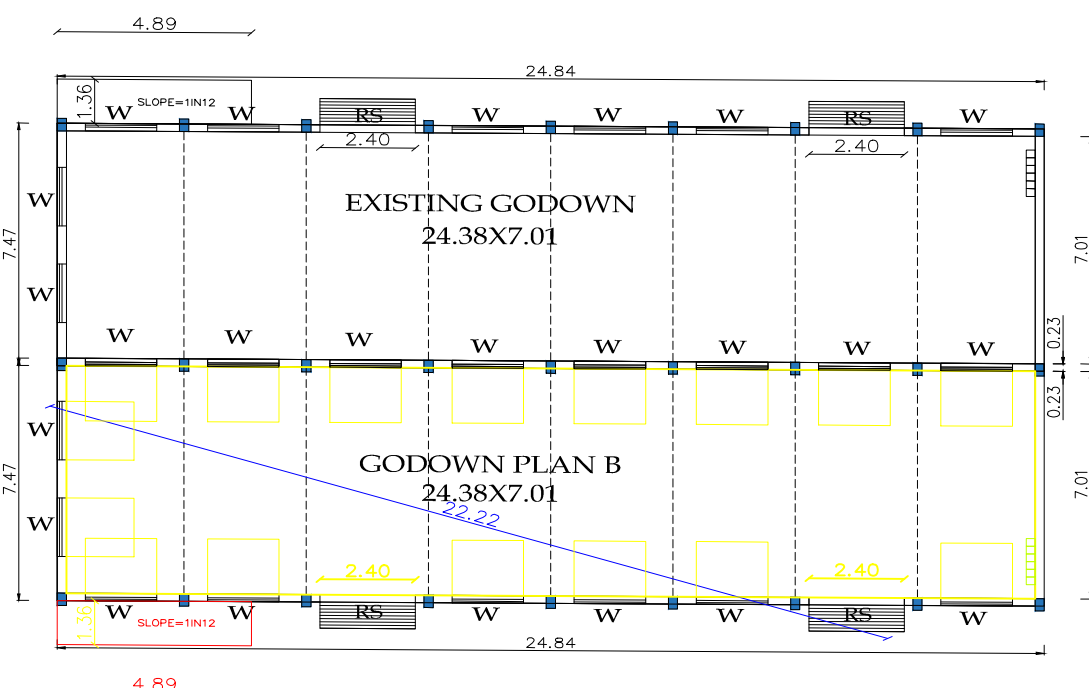
GROUND FLOOR
