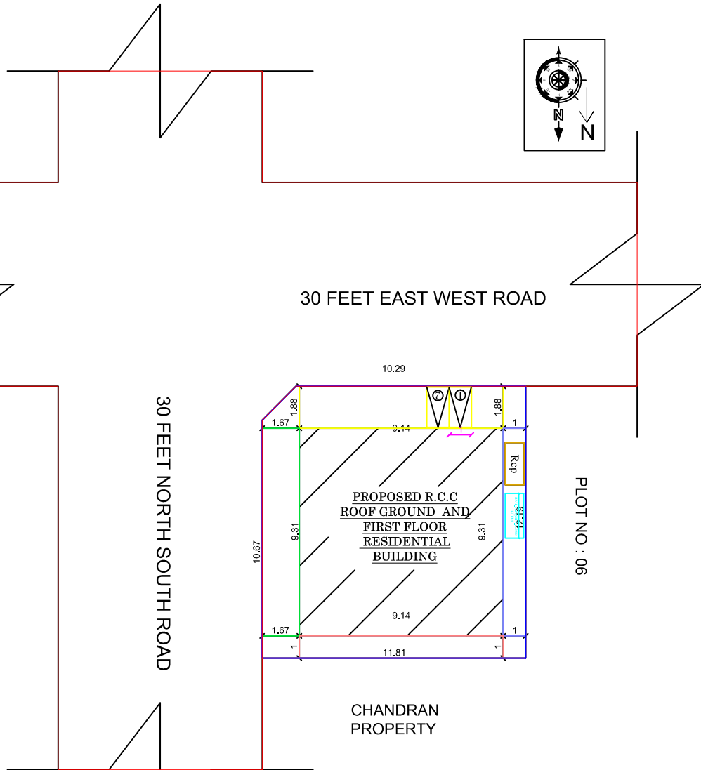
SITE PLAN
