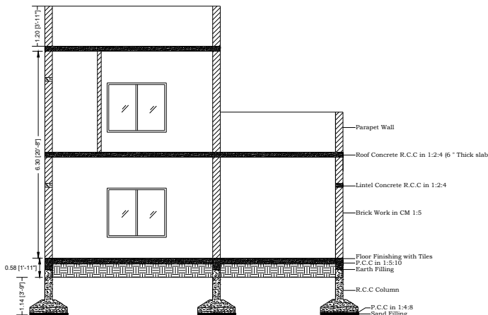
SECTION X-X
