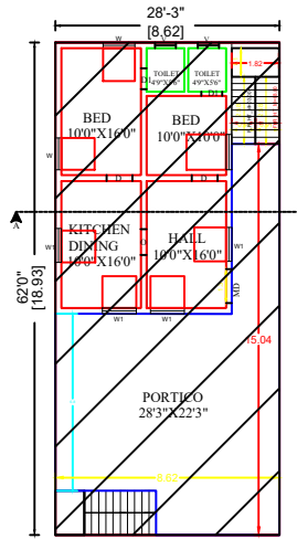
EXISTING GROUND FLOOR PLAN
