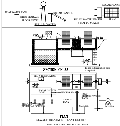
WASTE WATER RECYCLING UNIT
