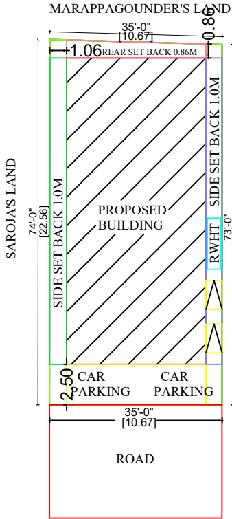
SITE PLAN
