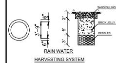
RAINWATER HARVESTING SYSTEM SCALE 1:50
