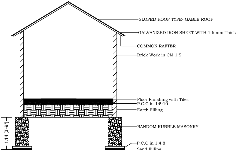
SECTION X-X
