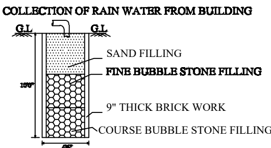
SECTION ON RAIN WATER COLLECTION TANK RAIN WATER COLLECTION TANK
