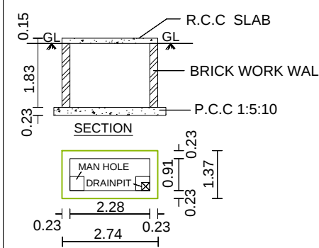
'SUMP_CAPACITY_L=6000' SUMP DETAILS
