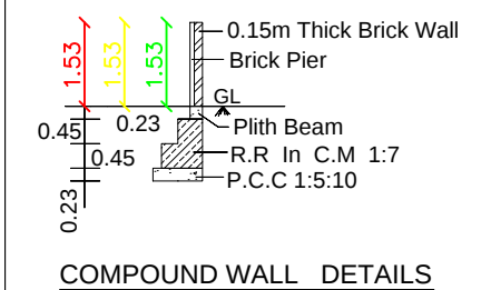
COMPOUND WALL DETAILS
