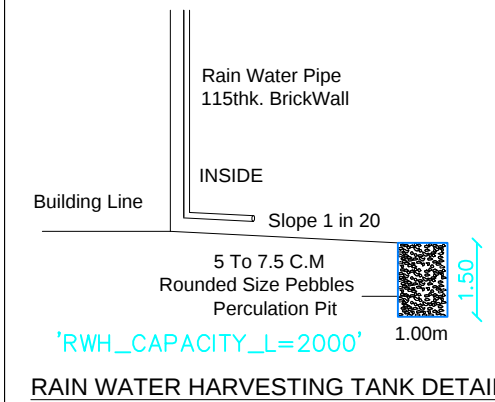
RAIN WATER HARVESTING TANK DETAILS
