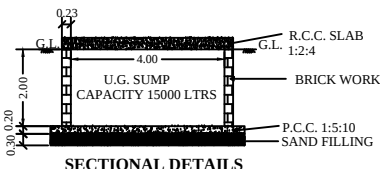
SUMP DETAILS
