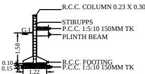
COLUMN DETAILS
