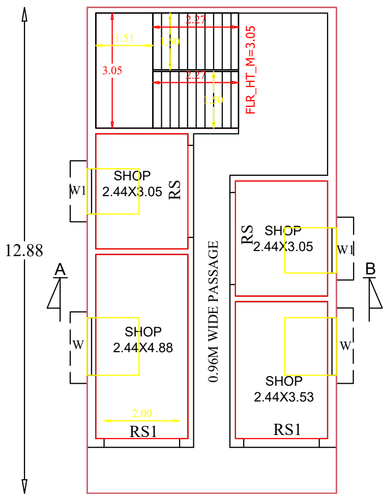
FRIST FLOOR PLAN SCALE 1 CM =1 M
