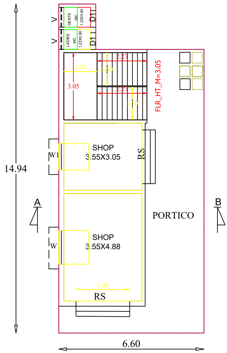
GROUND FLOOR PLAN SCALE 1 CM =1 M
