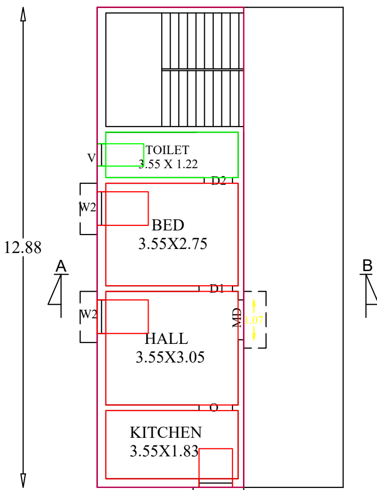
SECOND FLOOR PLAN SCALE 1 CM =1 M
