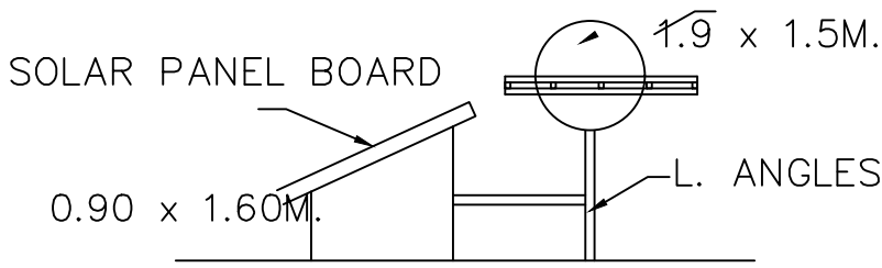
CROSS SECTION OF SOLAR WATER HEATING SYSTEM
