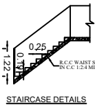
STAIRCASE DETAILS
