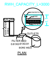
RAIN WATER HARVESTING SUMP
