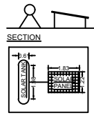
SOLAR SYSTEM
