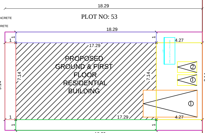
SITE PLAN
