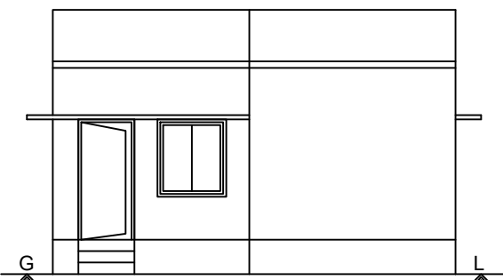
FRONT ELEVATION
