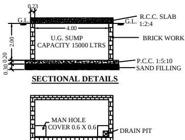
SUMP DETAILS
