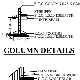
STAIR DETAILS
