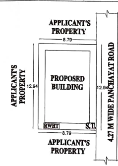
SITE PLAN SCALE = 1 : 500
