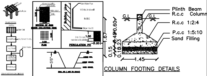
DETAILED PLAN OF RAINWATER PERCOLATION AND COLLECTION PIT
