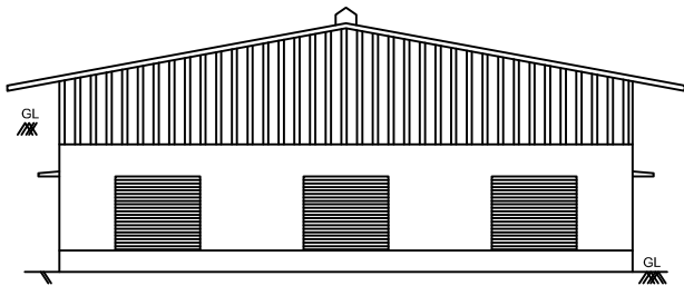
FRONT ELEVATION
