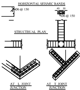
STRUCTURAL PLAN
