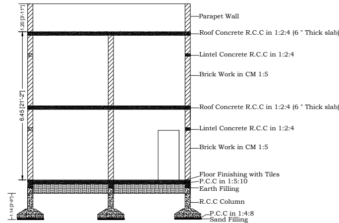
SECTION X-X
