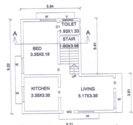
PLAN OF GROUND FLOOR
