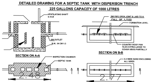
PLAN OF DISPERSION TRENCH
