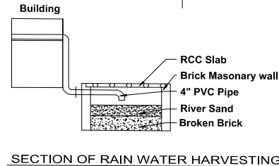
SECTION OF RAIN WATER HARVESTING
