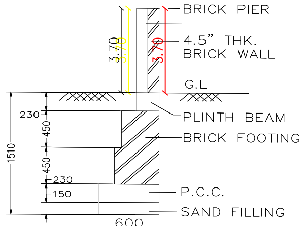
COMPOUND WALL DETAILS
