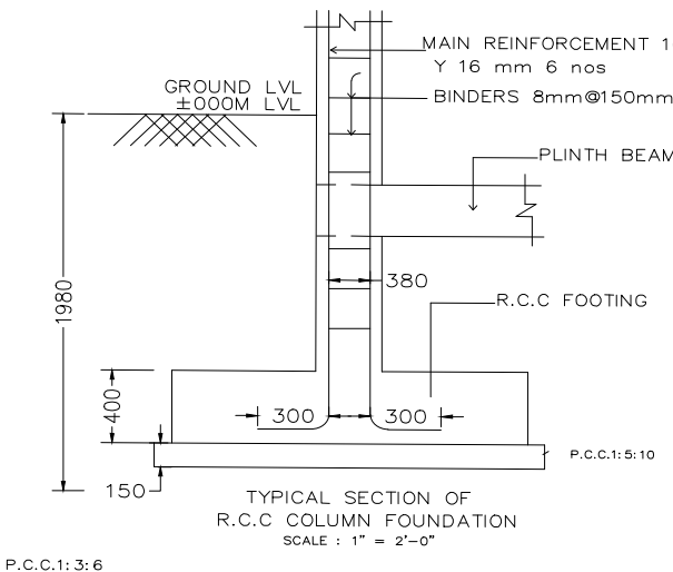
TYPICAL SECTION OF R.C.C COLUMN FOUNDATION
