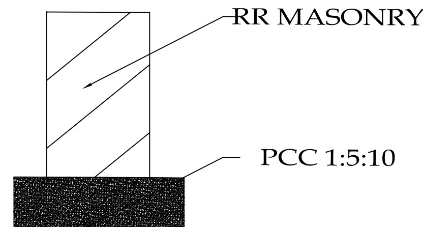
FOUNDATION DETAIL
