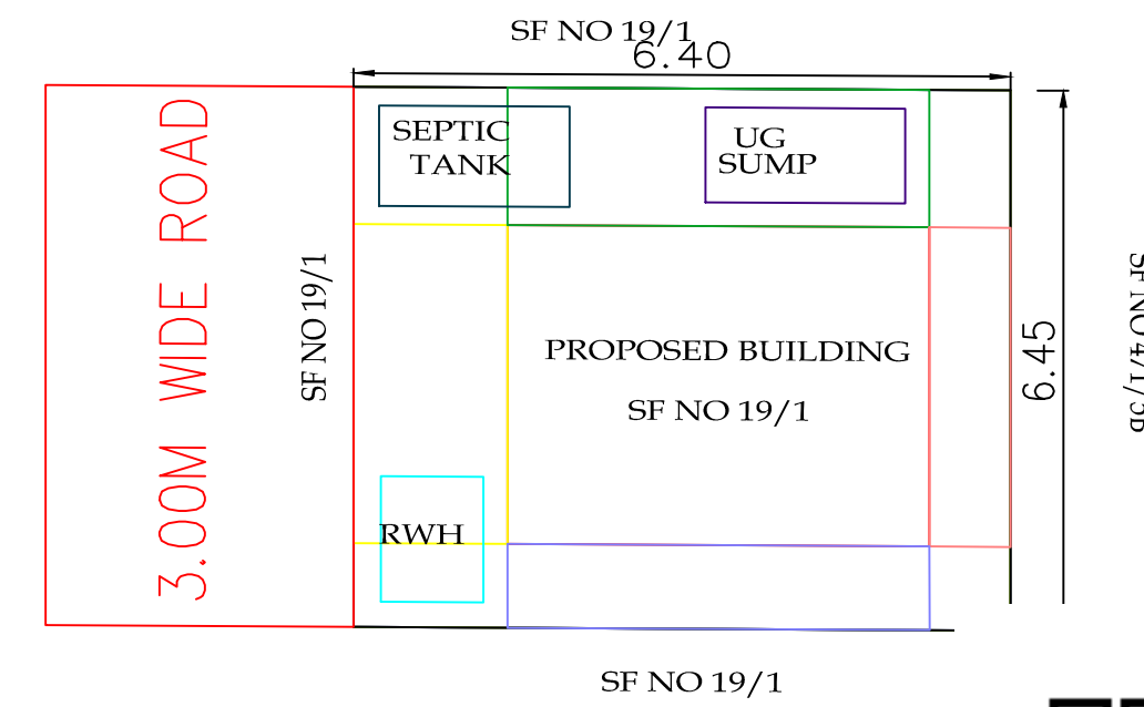
SITE PLAN
