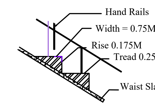
STAIRCASE DETAILS
