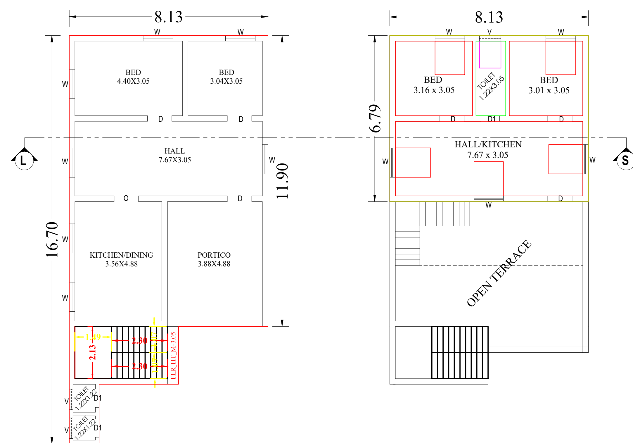
ADDITIONAL PROPOSED FIRST FLOOR PLAN SCALE 1:100
