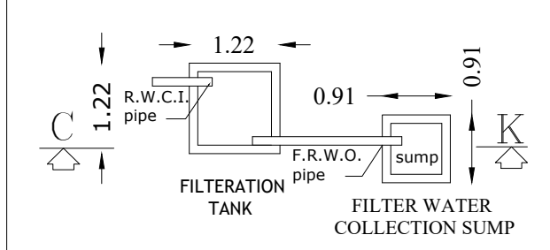
RAIN WATER STORAGE TANK PLAN (SCALE: 1cm=1m)
