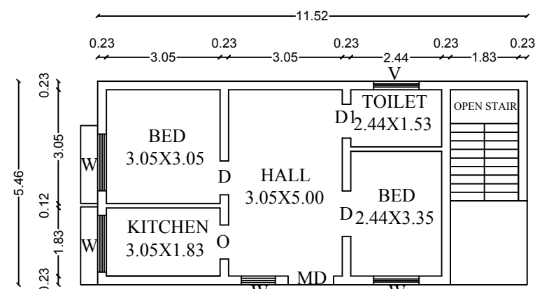
EXISTING GF.PLAN
