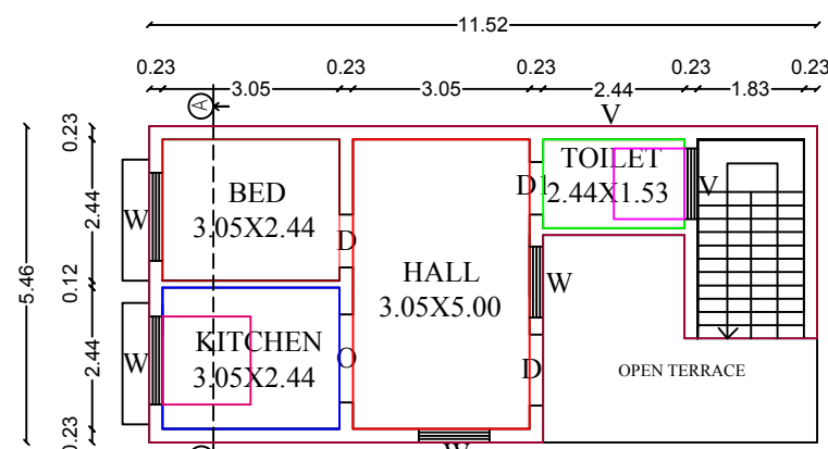
PROPOSED FF.PLAN
