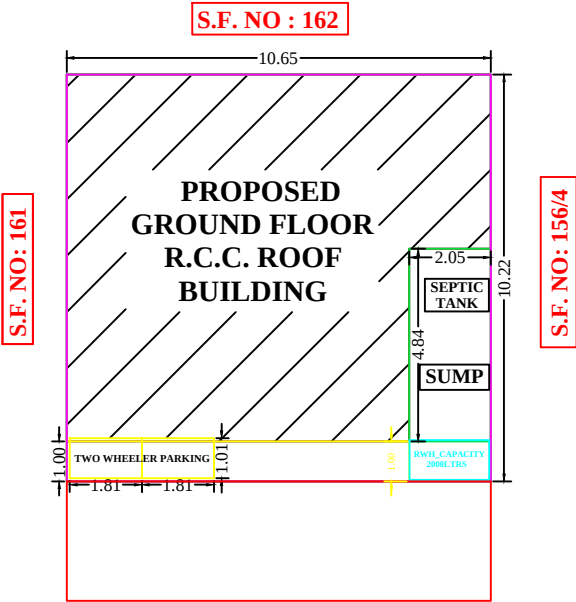
SITE PLAN
