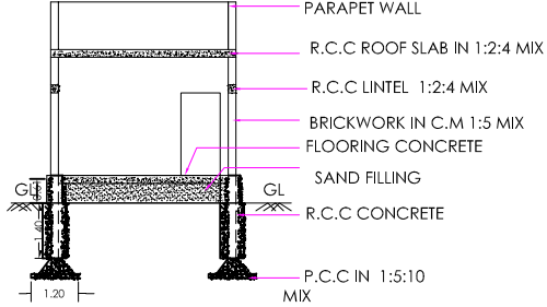
SECTION "AB"
