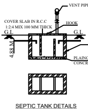
SEPTIC TANK DETAILS
