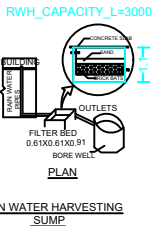
RAIN WATER HARVESTING SUMP
