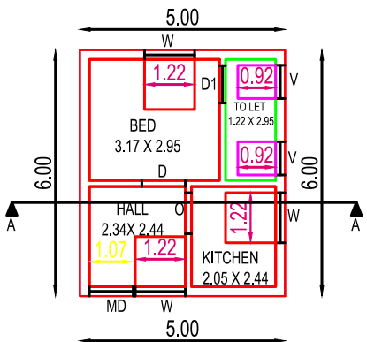
GROUND FLOOR PLAN (Scale 1:100)
