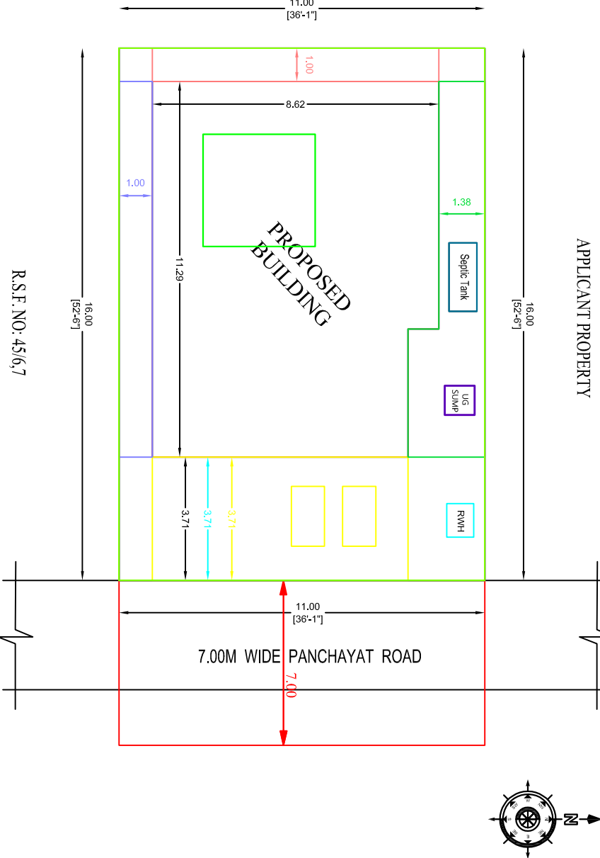
SITE PLAN (1:100)
