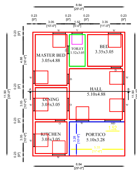
PROPOSED PLAN
