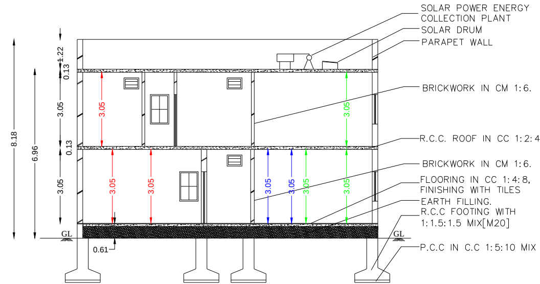
SECTION ON KK'
