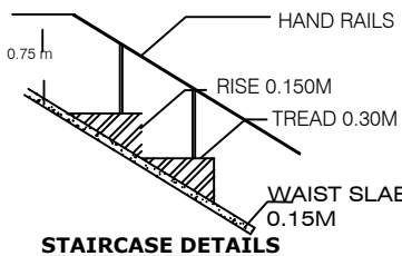
STAIRCASE DETAILS
