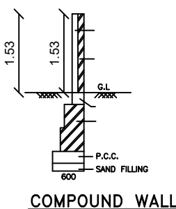
COMPOUND WALL
