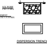
DISPERSION TRENCH
