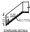
STAIRCASE DETAILS
