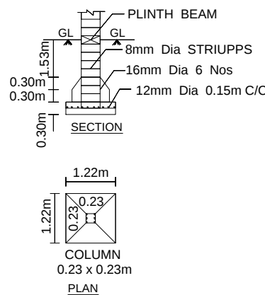
COLUMN FOUNDATION DETAILS
