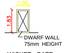
WICKET GATE
