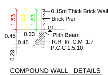
COMPOUND WALL DETAILS
