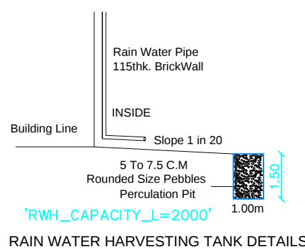
RAIN WATER HARVESTING TANK DETAILS
