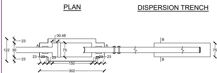
DESIGN OF SEPTIC TANK AND DISPERSION TRENCH CAPACITY : 1080 LITERS.
