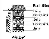
SECTION ON B-B.
