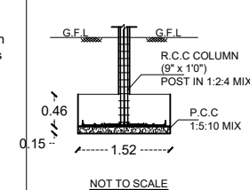
COLUMN POST DETAILS
