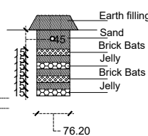
SECTION ON B-B.
