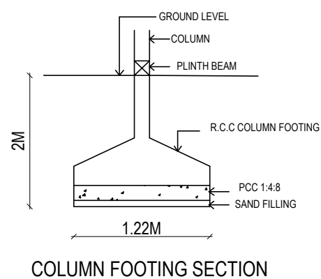
COLUMN FOOTING SECTION
