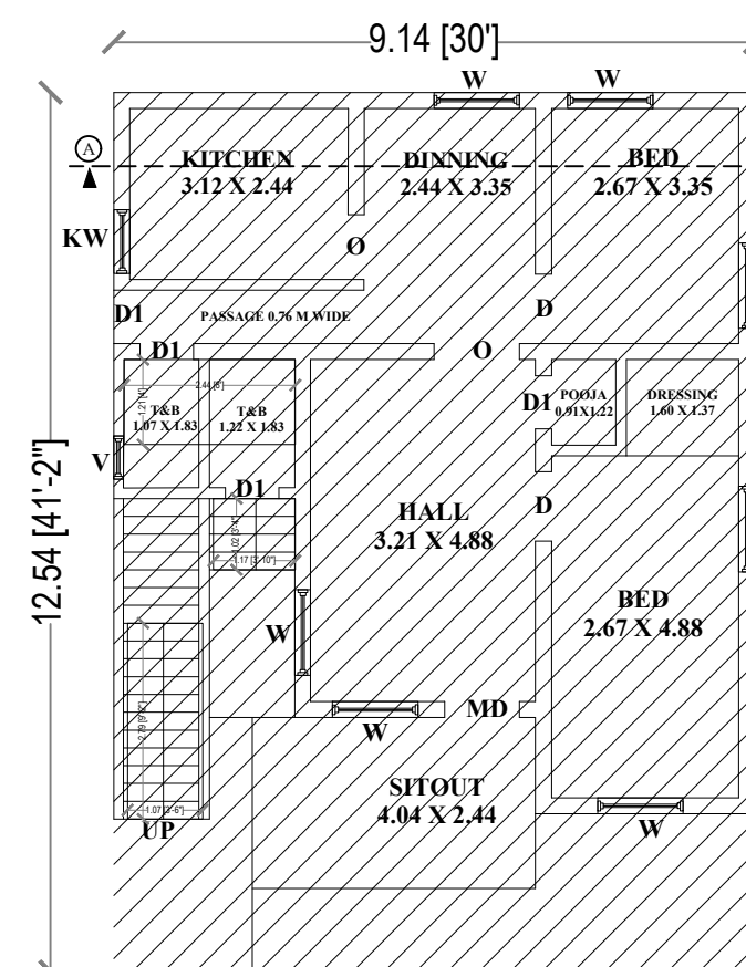
EXISTING GROUND FLOOR RCC & GI SHEET PLAN DOOR NO:130/3, ASS NO:2034.,
