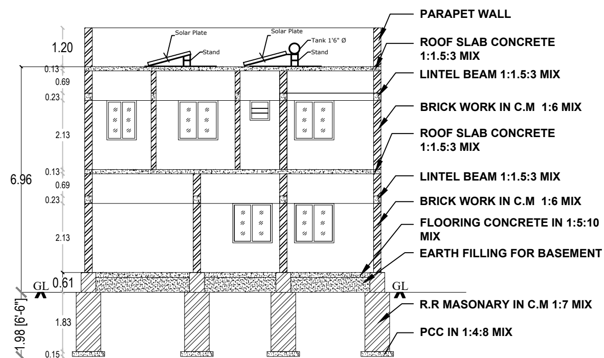
SECTION-'AB'
