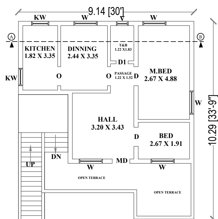
FIRST FLOOR RCC PLAN
