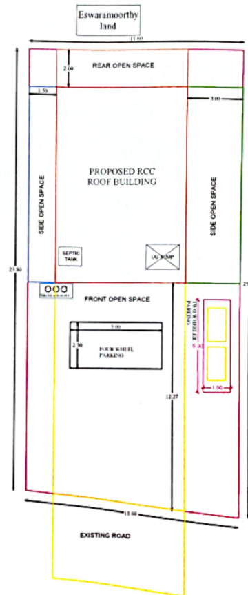
SITE & LOCATION PLAN SCALE - 1 : 700
