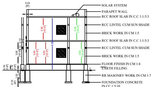
SECTION "AA","BB"
