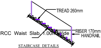
STAIRCASE DETAILS
