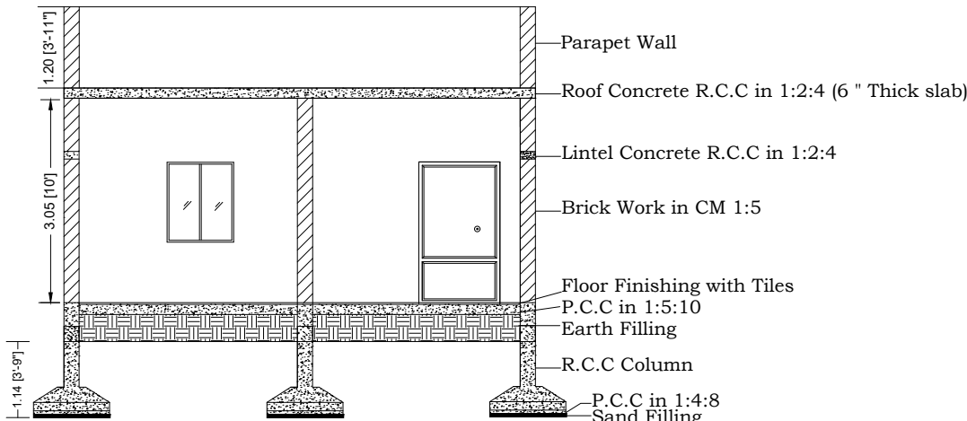
SECTION X-X
