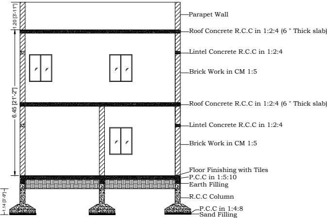
SECTION X-X
